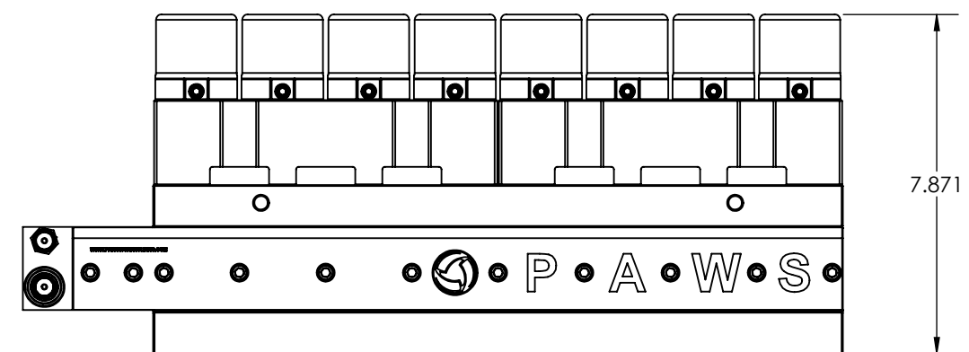
DA40 HYDRAULIC BASE 3080-40-CP
